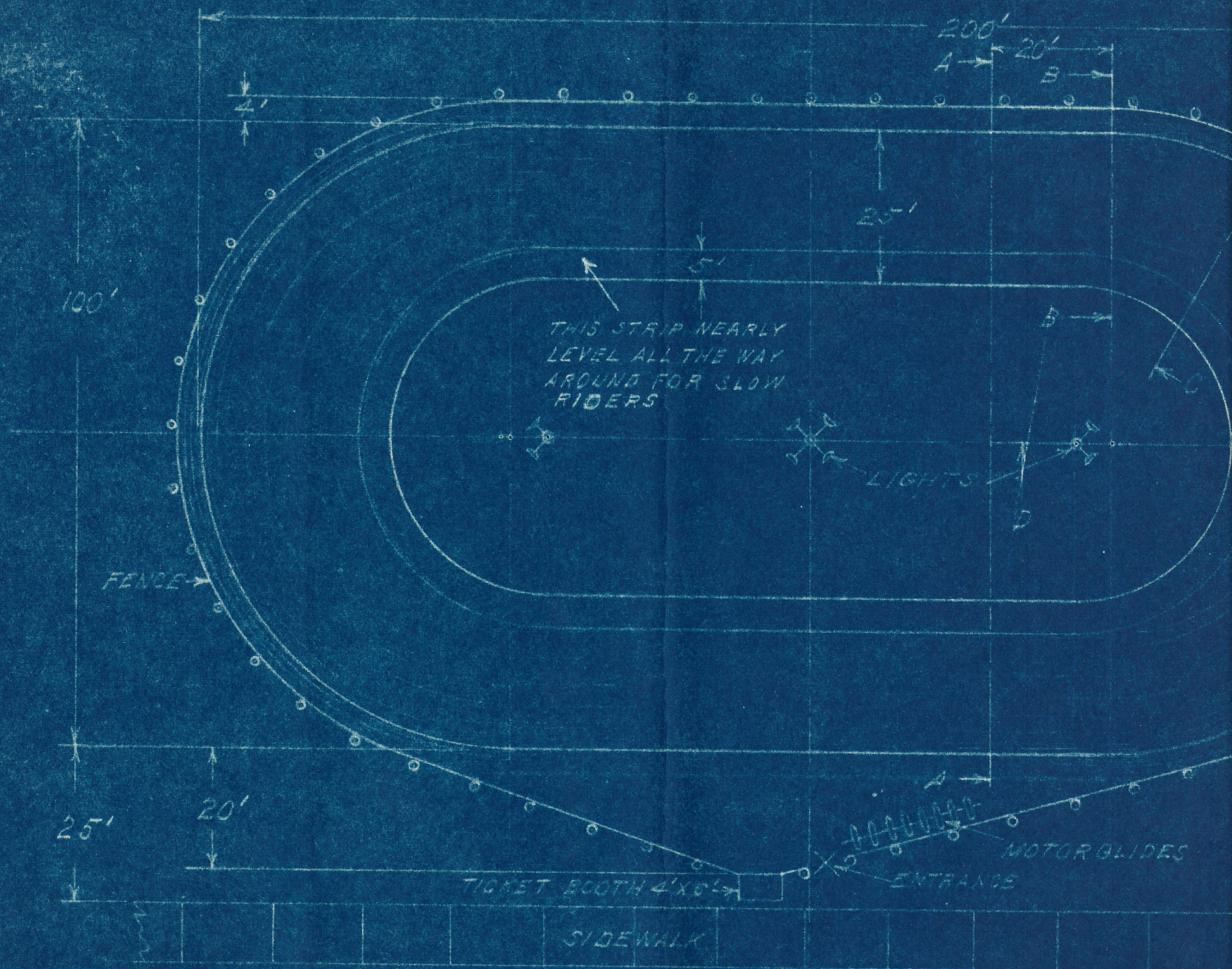
MOTOR GLIDE TRACK LAYOUT
