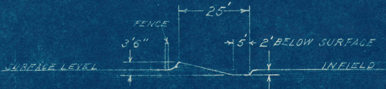
SEC. B-B SHOWING CONSTRUCTION OF TRACK AT BEGINNING OF TURN
