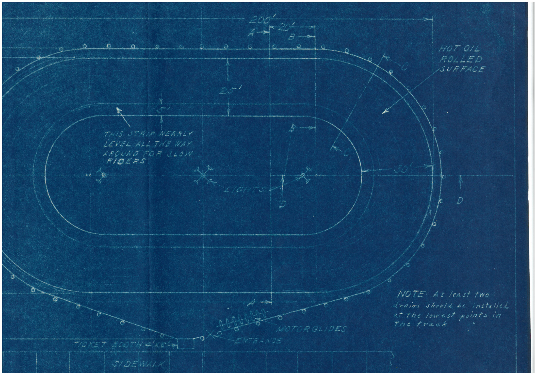
MOTOR GLIDE TRACK LAYOUT
