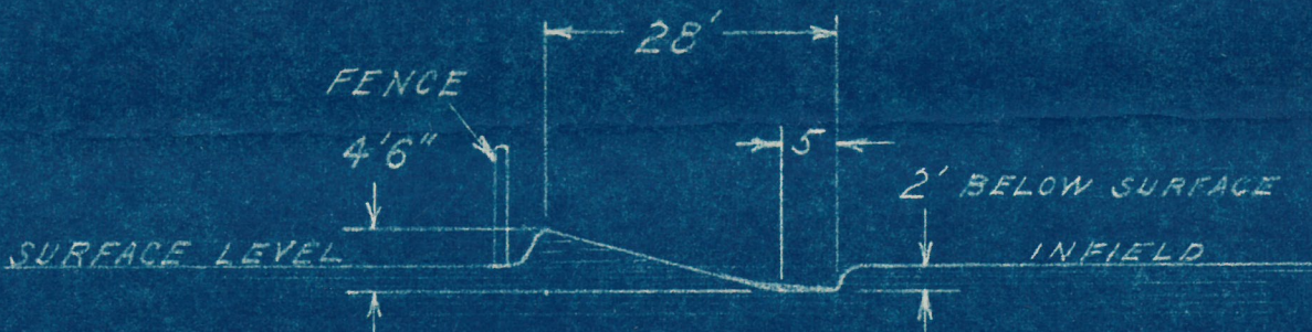
SEC. C-C SHOWING CONSTRUCTION OF TURN AT APPROXIMATELY 30° FROM BEGINNING OF TURN
