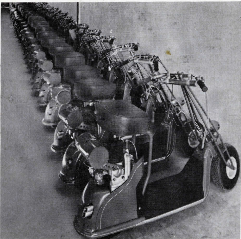
MOTOR GLIDES completed, tested and ready for shipment
